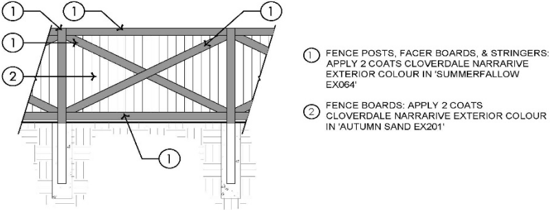
2 WOOD SCREEN FENCE COLOUR SCALE: 1:50
